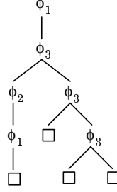
Fig. 4: A derivation tree in G_2 .
