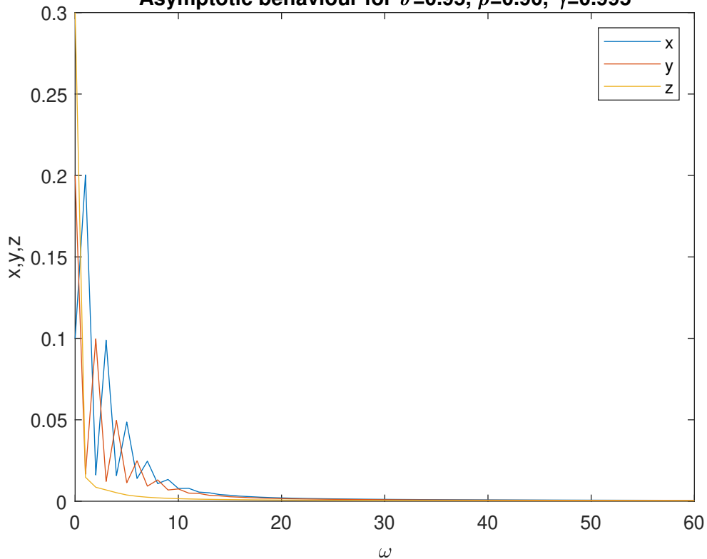
Asymptotic behaviour for \vartheta=0.95 , \rho=0.90 , \gamma=0.995
