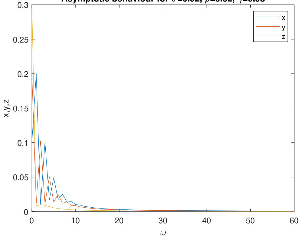
Asymptotic behaviour for \vartheta=0.92 , \rho=0.82 , \gamma=0.98
