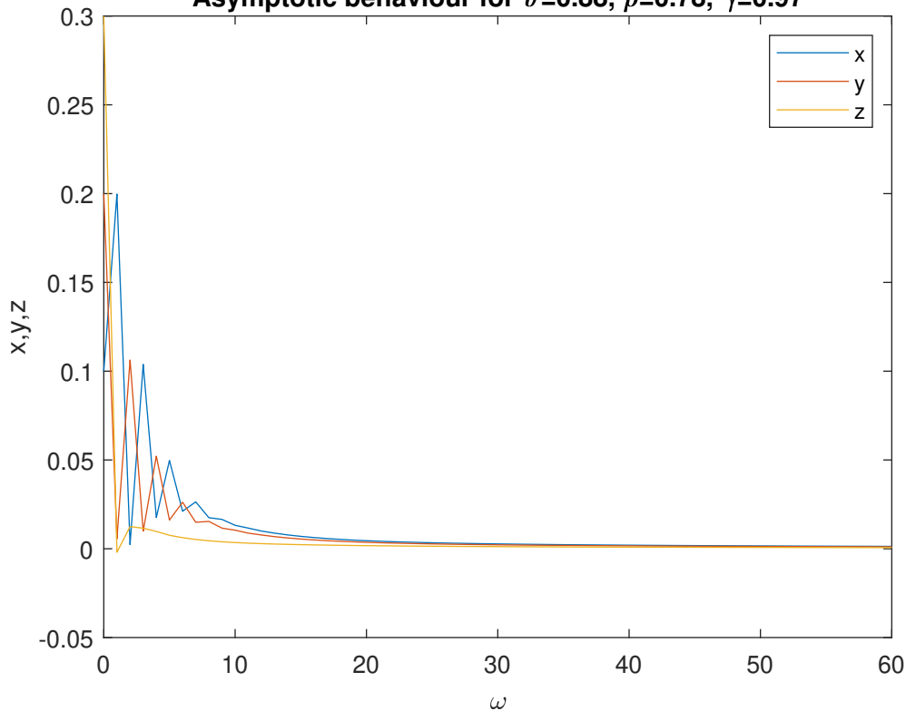
Asymptotic behaviour for \vartheta=0.88 , \rho=0.78 , \gamma=0.97
