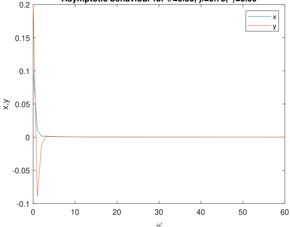
Asymptotic behaviour for \vartheta=0.95 , \rho=0.75 , \gamma=0.99
