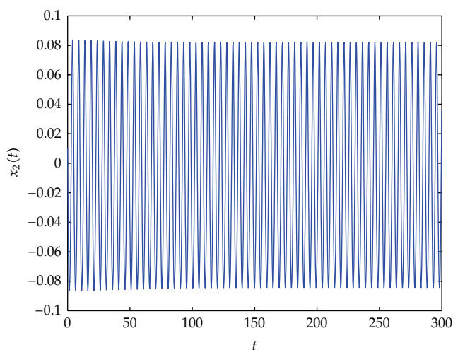
Figure 5: Trajectories graphs of the system (4.1) with \tau_1 = 0.01, \tau_2 = 0.04 , and \tau_1 + \tau_2 = 0.05 > \tau^0 \approx 0.01 . Hopf bifurcation occurs from the equilibrium E_*(0,0) . The initial value is (0.05, 0.01) .
