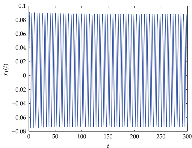
Figure 4: Trajectories graphs of the system (4.1) with \tau_1 = 0.01, \tau_2 = 0.04 , and \tau_1 + \tau_2 = 0.05 > \tau^0 \approx 0.01 . Hopf bifurcation occurs from the equilibrium E_*(0,0) . The initial value is (0.05, 0.01) .
