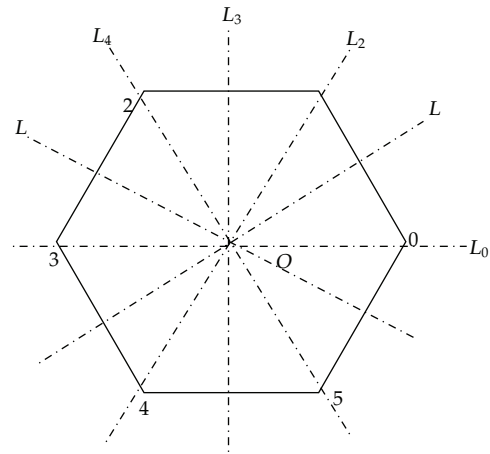
FIGURE 2: Regular 6 quadrature.
