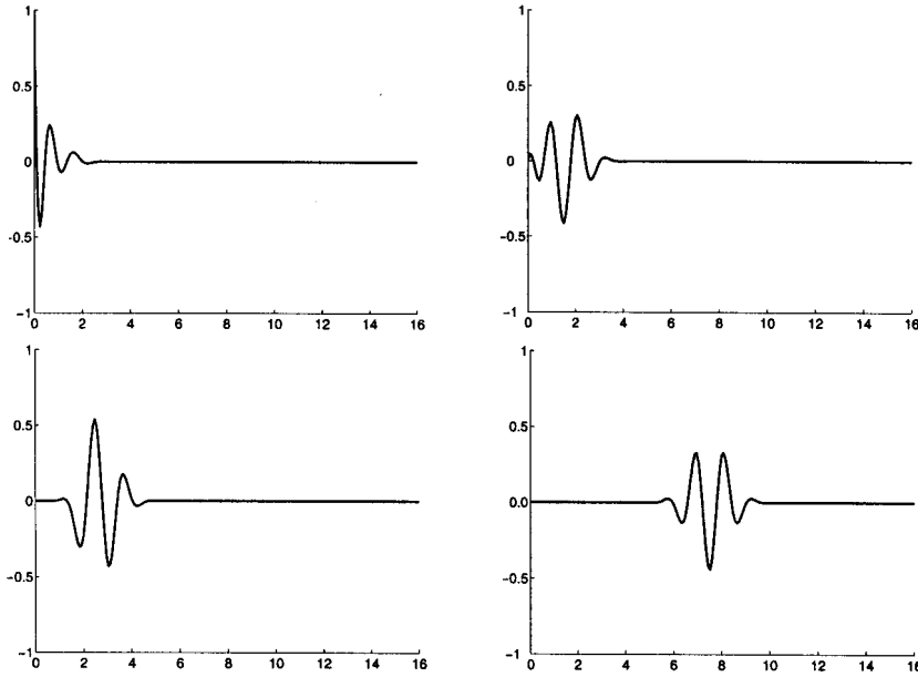
Fig. 4. Qubic spline-wavelets
