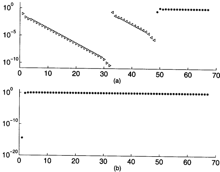
Fig. 6. Magnitude of wavelet and spline coefficients
