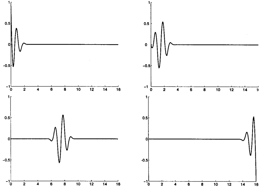
Fig. 3. Quadratic spline-wavelets
