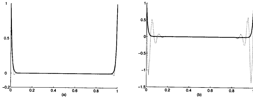
Fig. 8. The effect of the collocation points distribution in quadratic case
