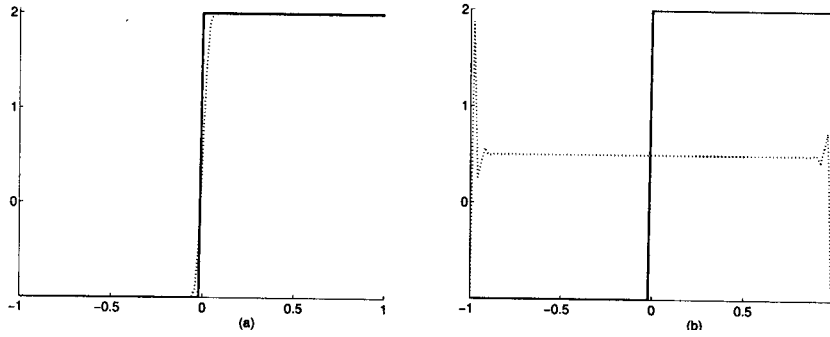
Fig. 7. The effect of the collocation points distribution in cubic case
