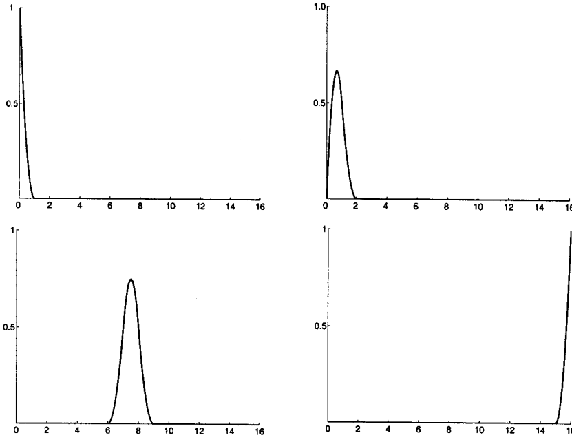
Fig. 1. Quadratic splines
