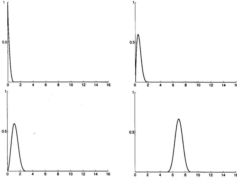
Fig. 2. Cubic splines
