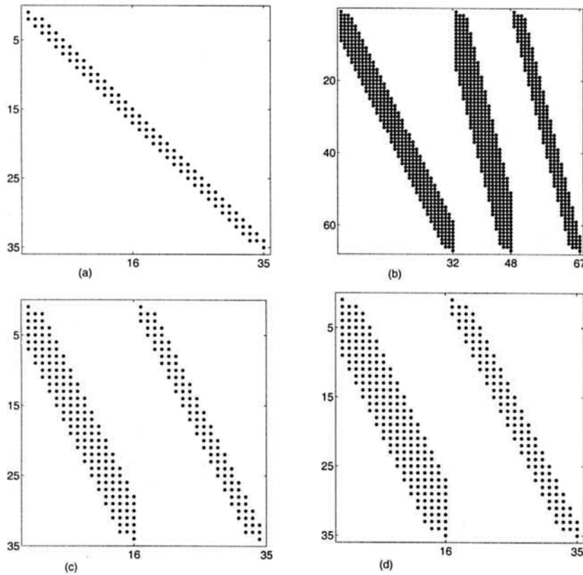
Fig. 5 Matrices assigned to spline and spline-wavelet bases
