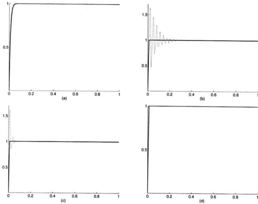
Fig. 9. The influence of small parameter and mesh size
