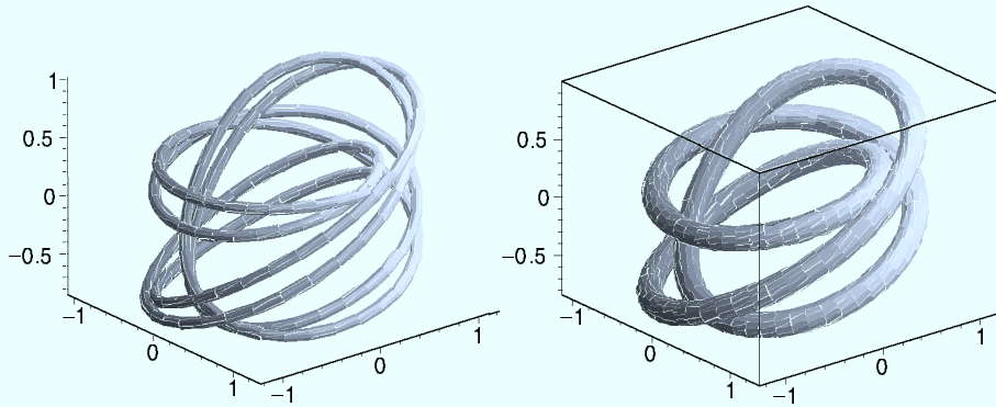
Figure 8. A cable knot, together with its companion torus knot, obtained using perturbation with M = 6 , j = 4 , k = 5 , w_j = 1 , w_k = 0.1 , \phi_j = \phi_k = \pi/2 , \rho_j = 0.2 , \rho_k = -0.3 and \epsilon = 0.02 .
