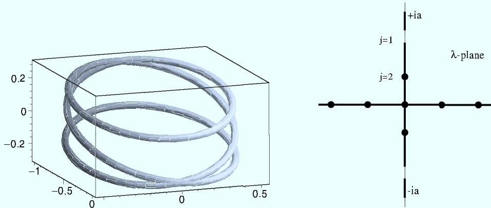
Figure 5. A self-intersecting curve arising from an even perturbation of a triply covered circle.
