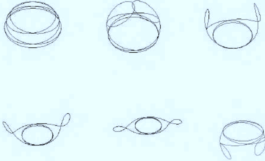
Figure 6. Time evolution frames of the Bäcklund transformation of a 5-fold planar circle.
