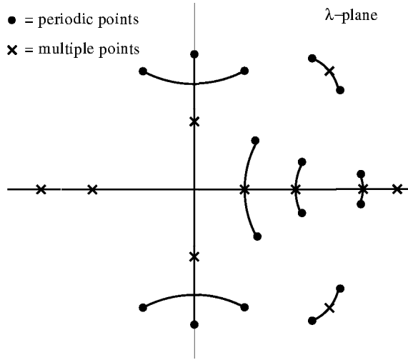
Figure 1. The Floquet spectrum of a typical NLS potential.
