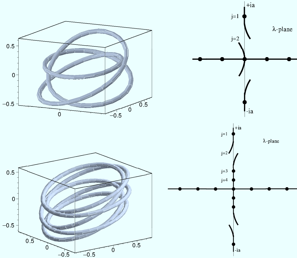
Figure 7. Above: a left-handed trefoil and its spectrum ( M = 3 , j = 2 , \rho = 0.2 , \phi = \pi/4 , \epsilon = 0.02 ). Below: a right-handed (5, 2) -torus knot and its spectrum ( M = 5 , j = 2 , \rho = -0.2 , \phi = \pi/4 , \epsilon = 0.1 )
